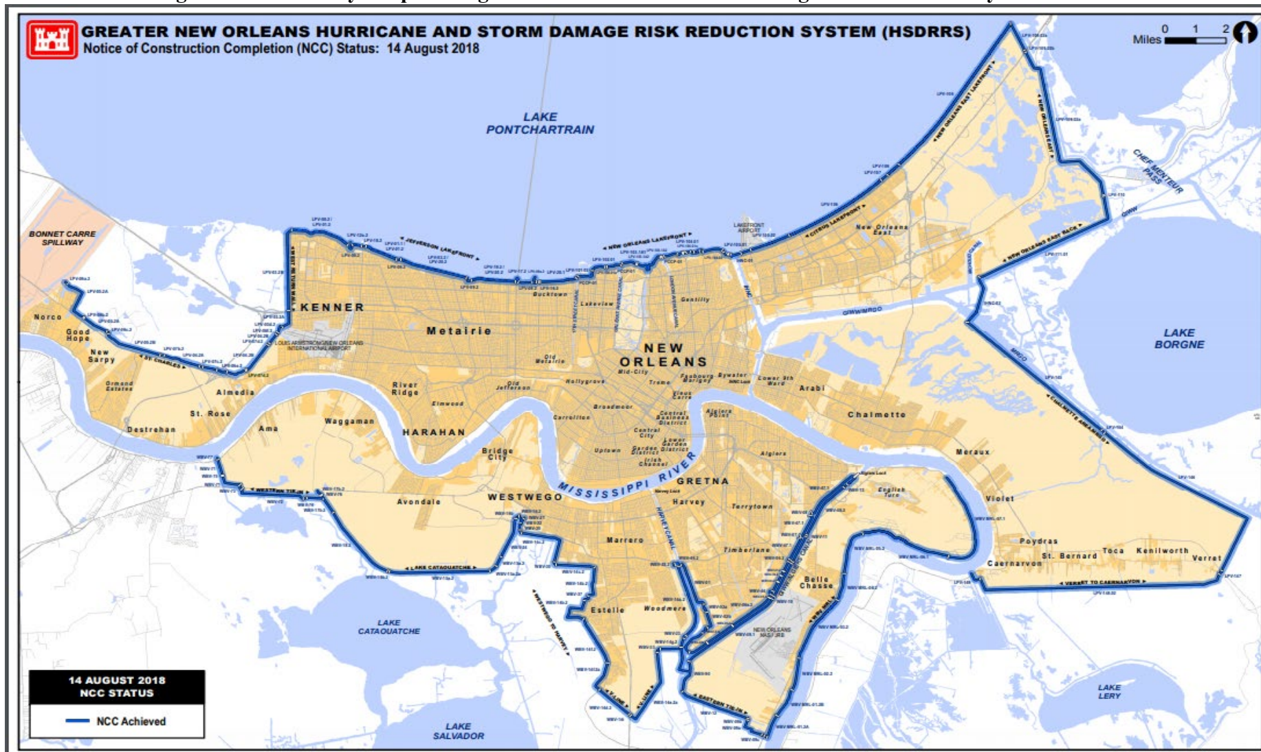
Figure 50: U.S. Army Corps of Engineers Hurricane & Storm Damage Risk Reduction System
